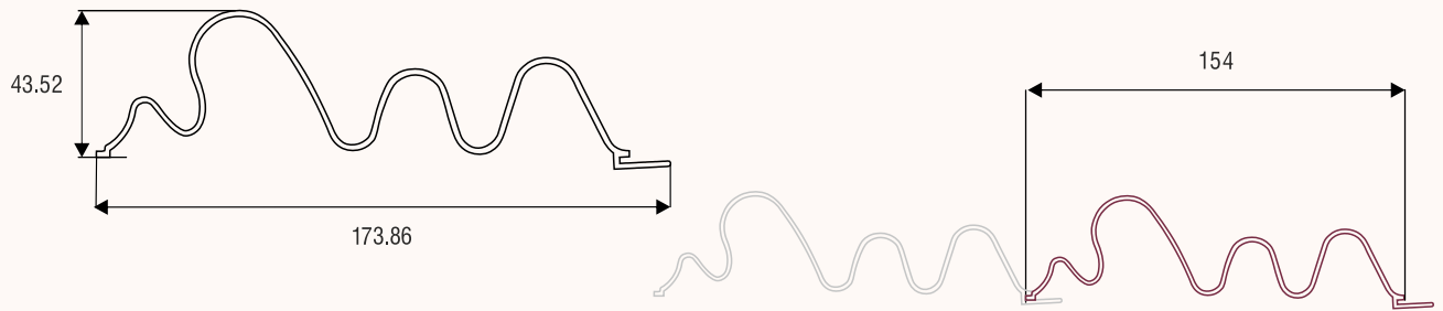
Adjoining Panel Placement
