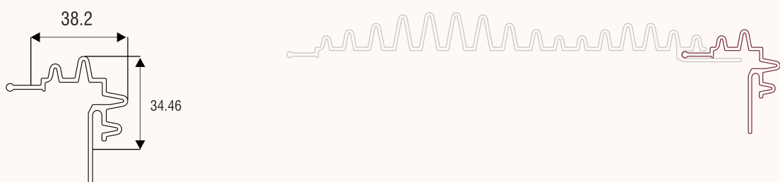
Outer Profile Placement
