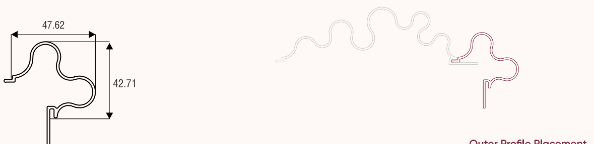
Outer Profile Placement
