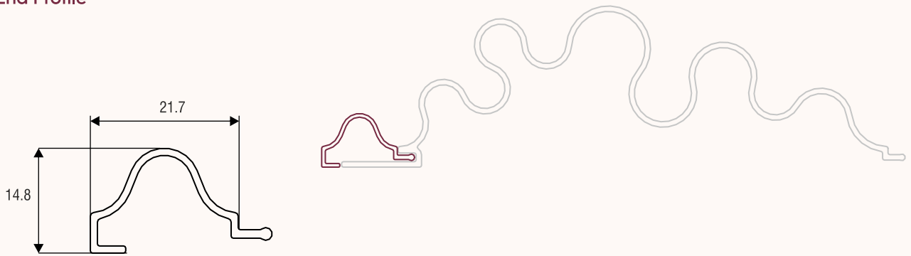
End Profile Placement
