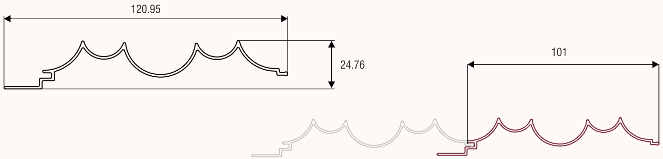
Adjoining Panel Placement
