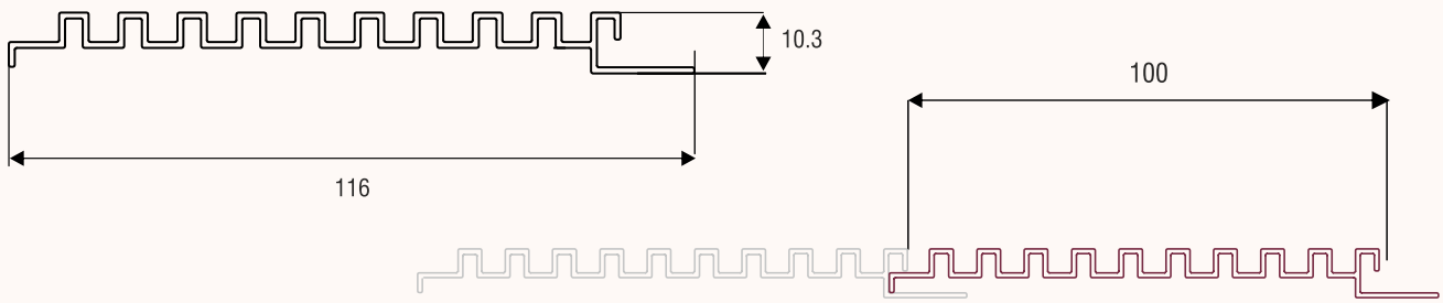
Adjoining Panel Placement
